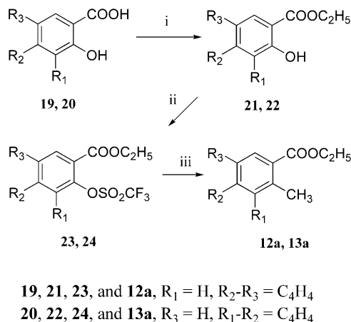
Scheme 4. Reagents: (i) (a) \text{SOCl}_2 ; (b) EtOH, \text{Et}_3\text{N} ; (ii) (\text{CF}_3\text{SO}_2)_2\text{O} , \text{C}_3\text{H}_5\text{N} ; (iii) (\text{CH}_3)_4\text{Sn} , LiCl, \text{Pd}(\text{PPh}_3)_2\text{Cl}_2 , DMF.
