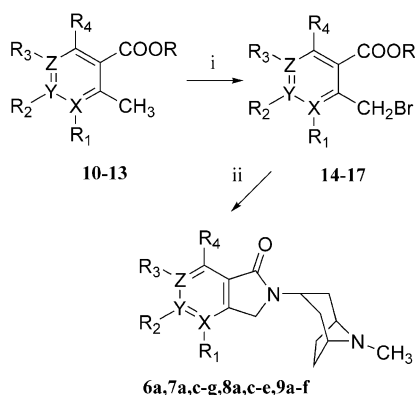
Scheme 1. Reagents: (i) NBS, dibenzoyl peroxide, \text{CCl}_4 ; (ii) endo -8-methyl-8-azabicyclo[3.2.1]oct-3-ylamine, EtOH.
