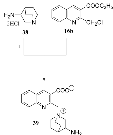
Scheme 9. Reagents: (i) \text{Na}_2\text{CO}_3 , \text{EtOH} .
