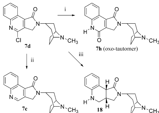
Scheme 3. Reagents: (i) HCl; (ii) \text{H}_2 (14 psi), Pd/C, \text{Et}_3\text{N} , EtOH; (iii) \text{H}_2 (50 psi), Pd/C, \text{Et}_3\text{N} , EtOH.
