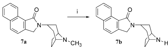
Scheme 2. Reagents: (i) \alpha -chloroethyl chloroformate (ACE-Cl).
