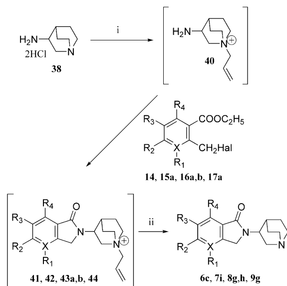
Scheme 10. Reagents: (i) (a) \text{Na}_2\text{CO}_3 , \text{EtOH} , (b) \text{CH}_2=\text{CHCH}_2\text{Br} ; (ii) (\text{CH}_3\text{CH}_2\text{CH}_2)_2\text{NH} , \text{Pd}(\text{PPh}_3)_2\text{Cl}_2 , \text{DMF} .
