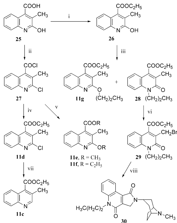
Scheme 5. Reagents: (i) (a) \text{SOCl}_2 ; (b) EtOH, \text{Et}_3\text{N} ; (ii) \text{POCl}_3 ; (iii) (a) NaH, DMF; (b) \text{CH}_3(\text{CH}_2)_2\text{I} ; (iv) EtOH, \text{Et}_3\text{N} ; (v) NaH, ROH; (vi) NBS, dibenzoyl peroxide, \text{CCl}_4 ; (vii) \text{H}_2 (14 psi), Pd/C, \text{Et}_3\text{N} , EtOH; (viii) endo -8-methyl-8-azabicyclo[3.2.1]oct-3-ylamine, EtOH.
