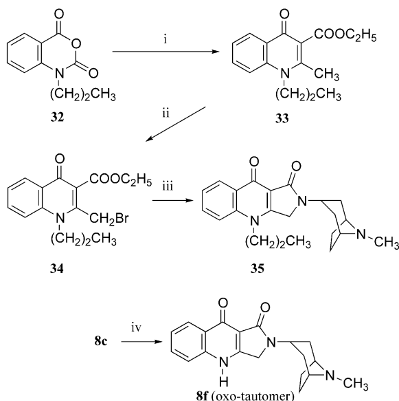
Scheme 7. Reagents: (i) \text{CH}_3\text{-CO-CH}_2\text{-COOC}_2\text{H}_5 , \text{NaH} , \text{DMA} ; (ii) \text{NBS} , dibenzoyl peroxide, \text{CCl}_4 ; (iii) endo -8-methyl-8-azabicyclo[3.2.1]oct-3-ylamine, \text{EtOH} ; (iv) \text{HCl} .
