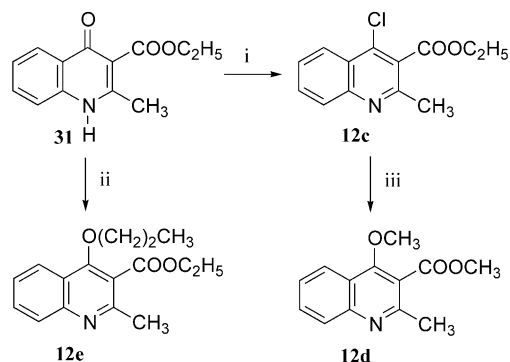
Scheme 6. Reagents: (i) \text{POCl}_3 ; (ii) (a) \text{NaH} , \text{DMF} ; (b) \text{CH}_3(\text{CH}_2)_2\text{I} ; (iii) \text{NaH} , \text{MeOH} .
